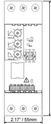
Mounting Centers 1.57" (40mm) x 6.10" (155mm)
