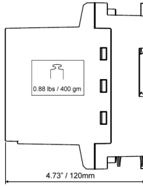
Mounting Centers 1.18" (30mm) x 5.2" (130mm)
