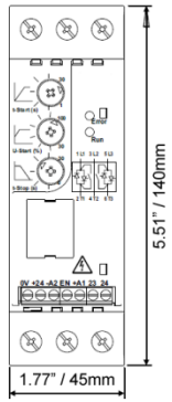
Mounting Centers 1.18" (30mm) x 5.2" (130mm)
