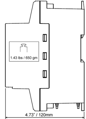
Mounting Centers 1.57" (40mm) x 6.10" (155mm)
